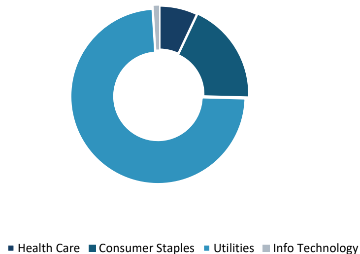
Sector Contribution to Emissions
