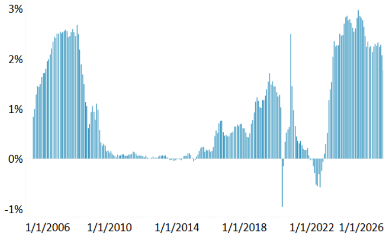
Rolling 6-Month Total Returns (Net of Fees)
