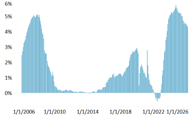
Rolling 12-Month Total Returns (Net of Fees)
